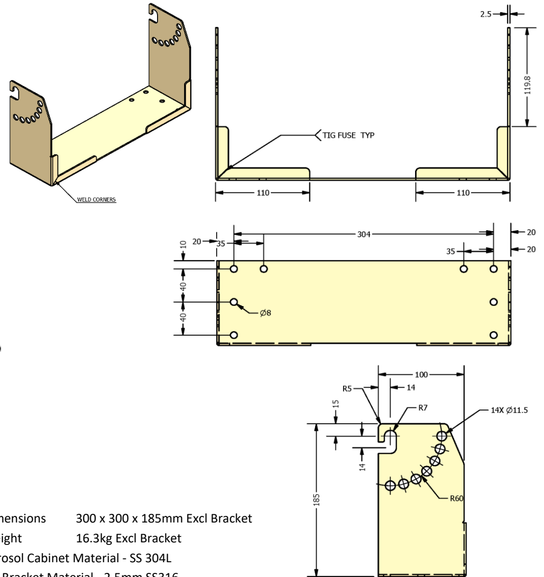
HD Bracket - FP-6100 shown
